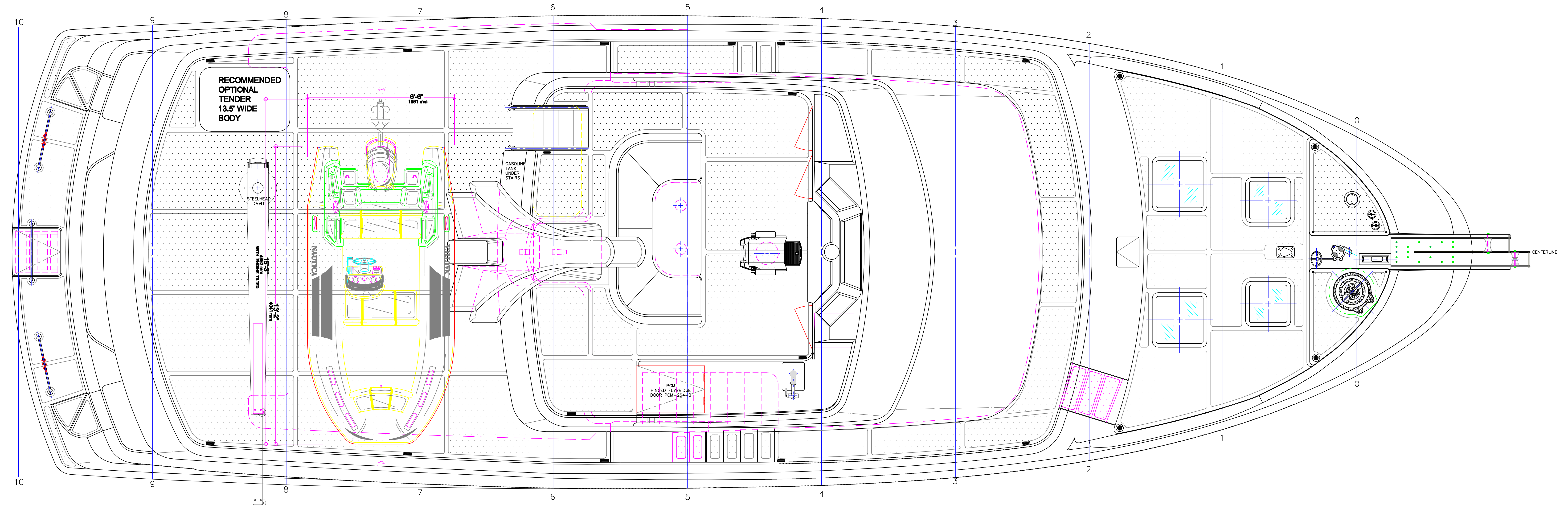
DECK PLAN 1/2"=1'-0"
