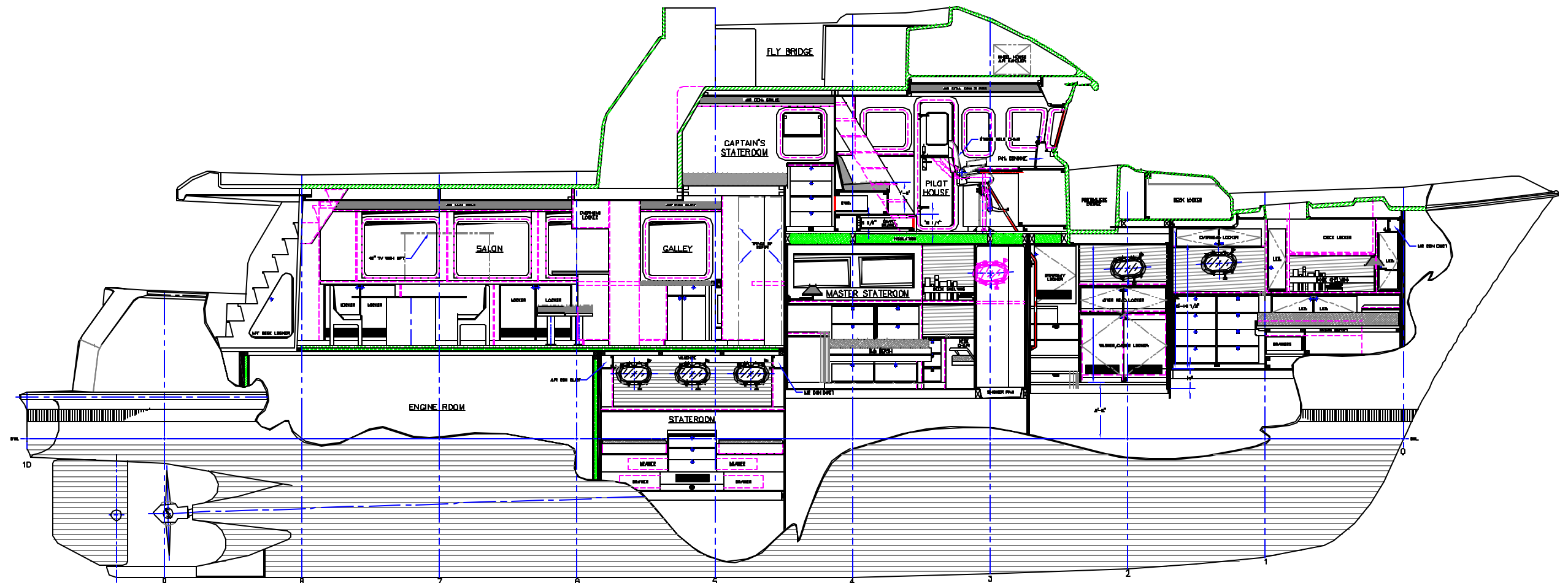
PORT INTERIOR PROFILE SECTION 1/2"=1'-0"
