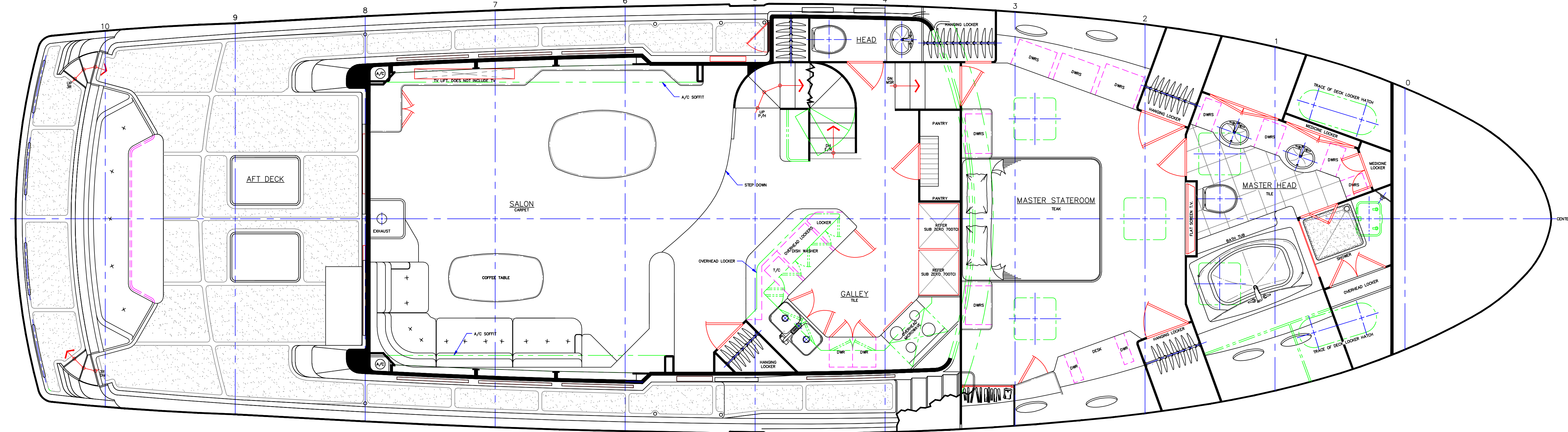
AFT PILOT HOUSE INTERIOR PLAN
