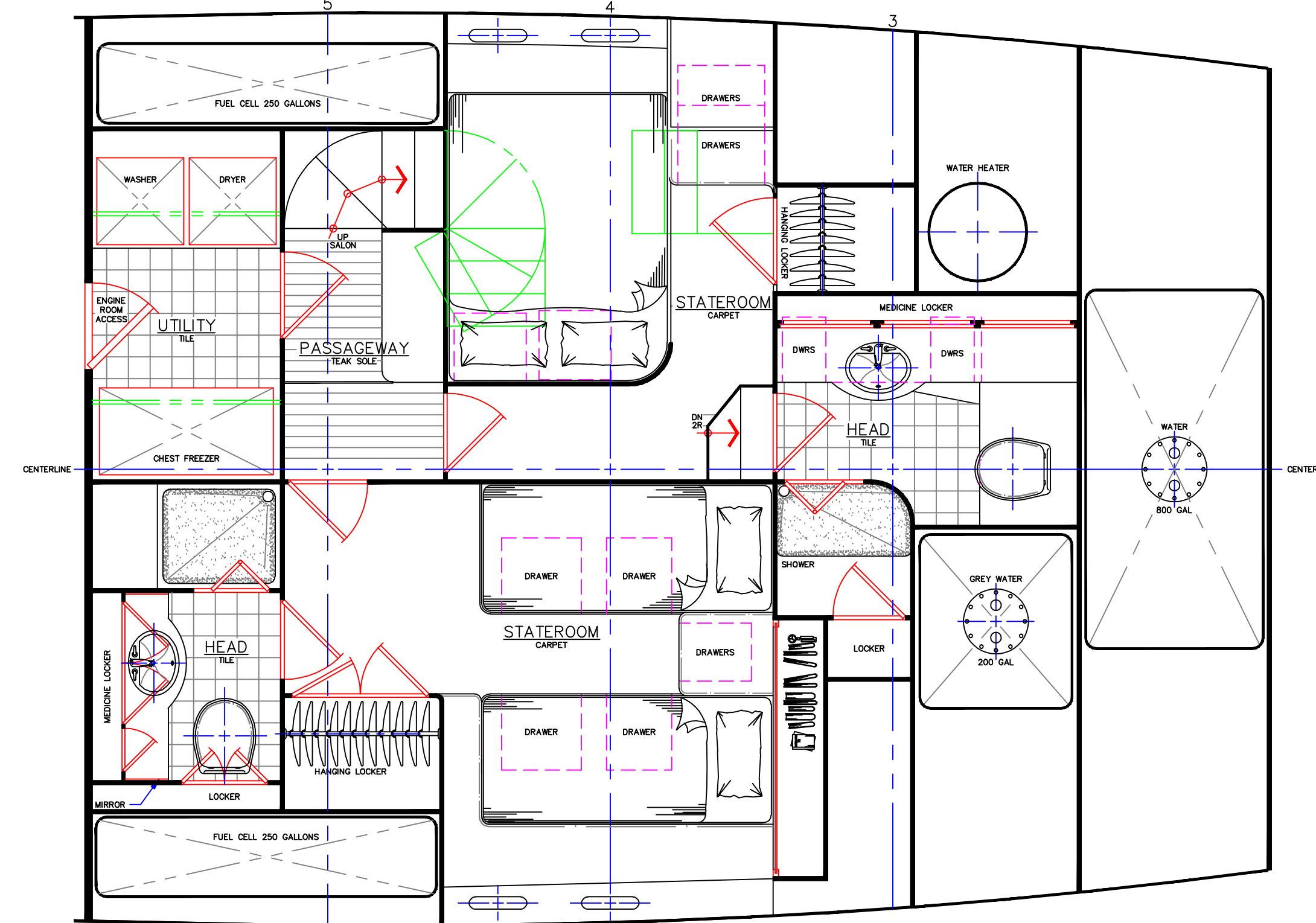
STATEROOMS (LOWER DECK)
