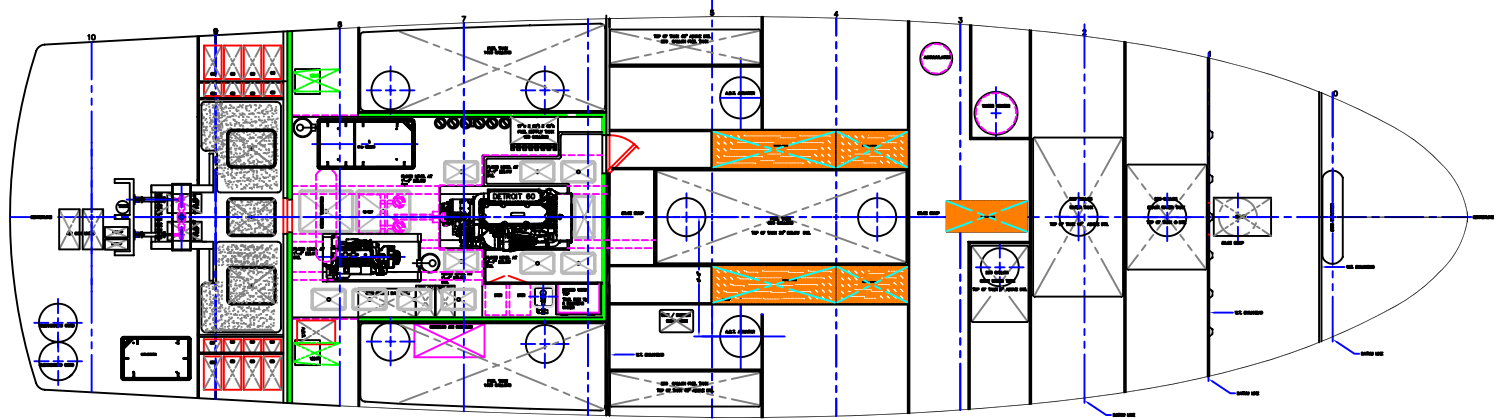
MACHINERY AND TANKAGE PLAN
