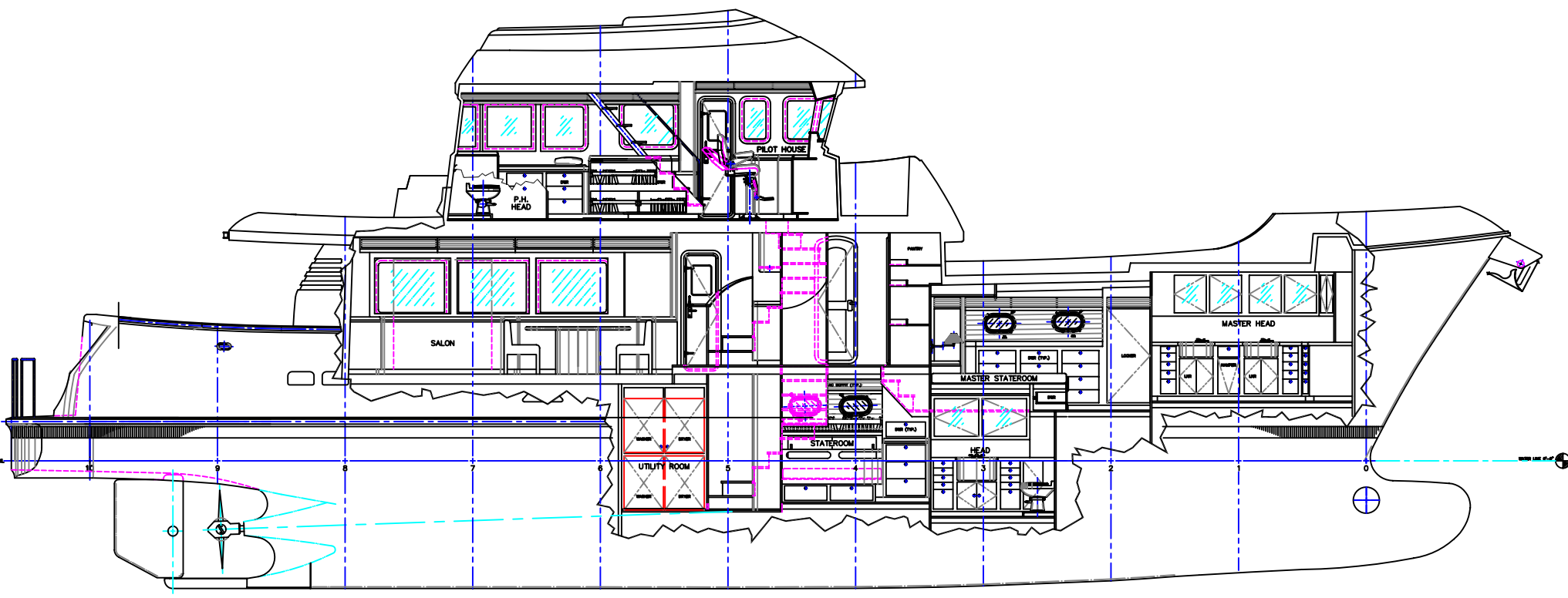
AFT PILOT HOUSE PORT INTERIOR PROFILE 1/2"=1'-0"
