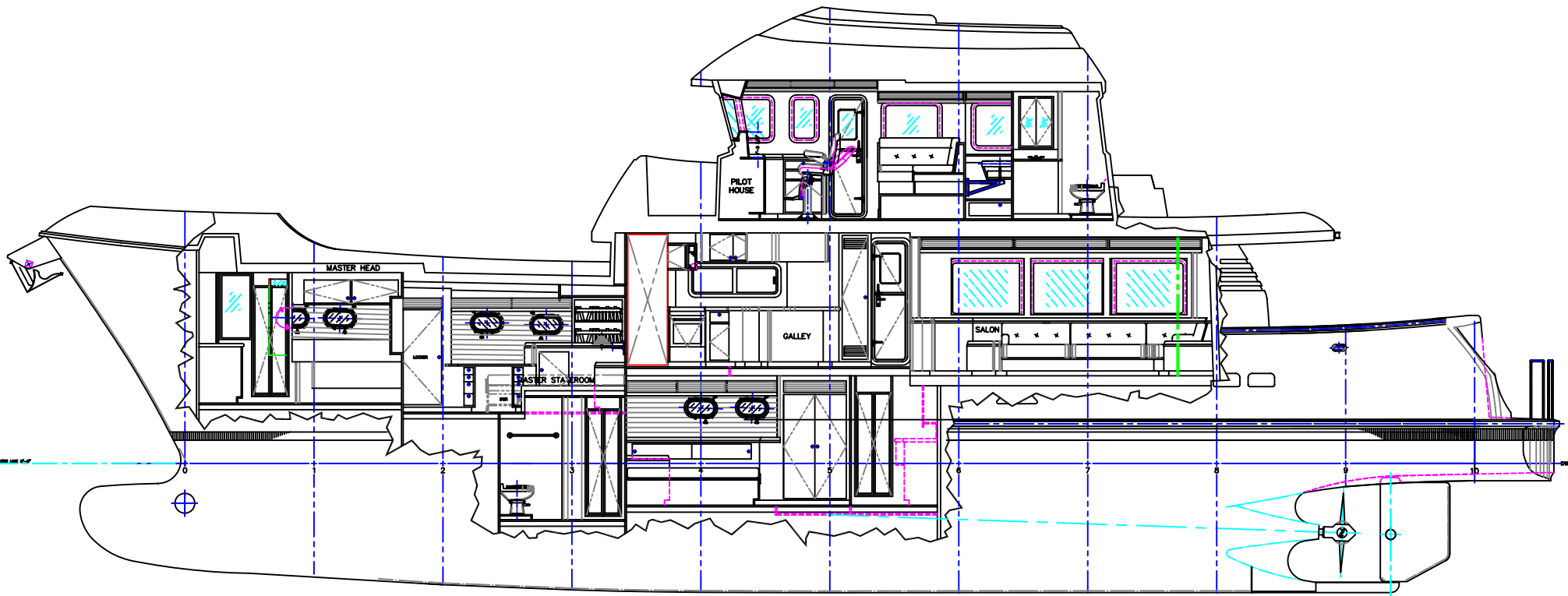
AFT PILOT HOUSE STARBOARD INTERIOR PROFILE 1/2"-0"
